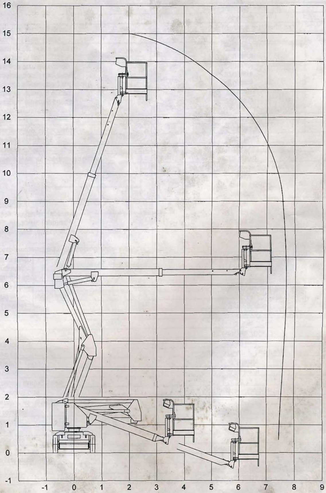
Fig. 3 - Working area
